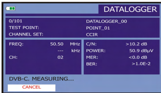
Figure 12.- DATALOGGER screen.
