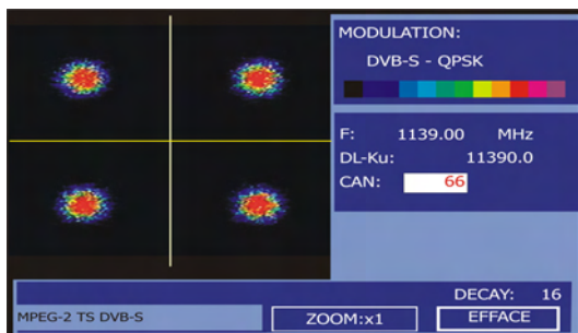
Figure 44.- Diagramme de constellation. Signal DVB-S (QPSK).
