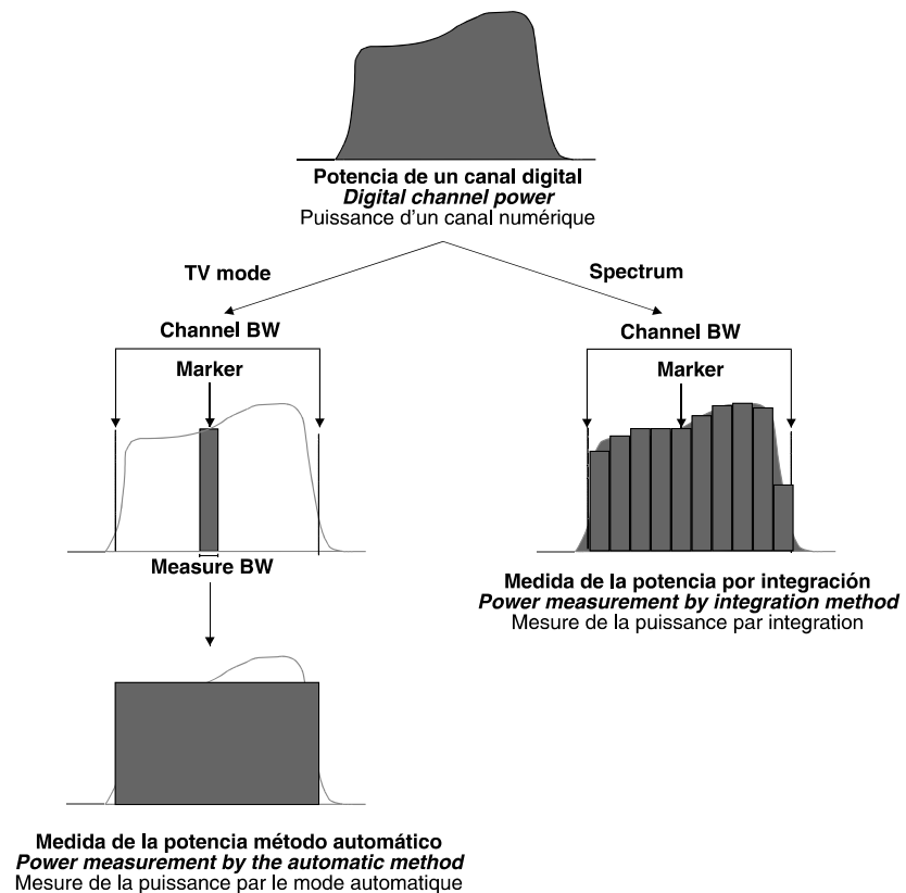
Figure 11.- Measuring digital power.
