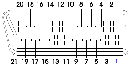
Figure 72.- Scart socket (external view).
