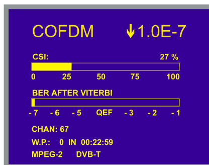
Figure 15.- BER measuring screen for COFDM-modulated signals
