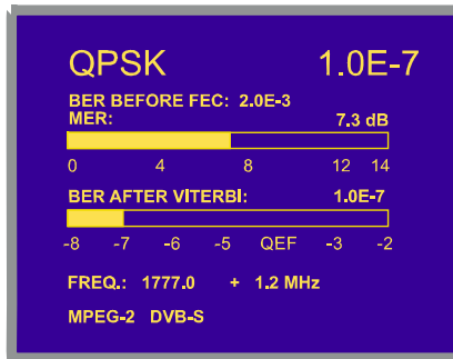
Figure 19.- BER measuring screen for QPSK modulated signals.
