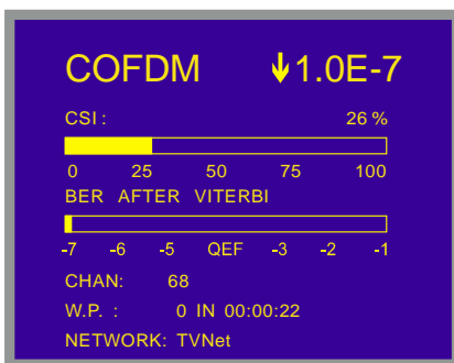
Figure 36.- Tuning a digital channel with acceptable BER level.
