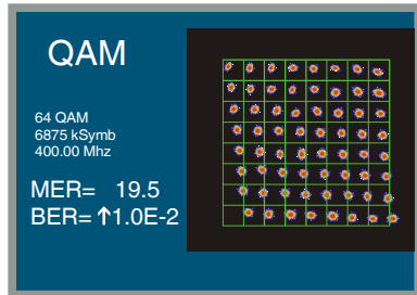
Figure 28.- Signal with phase error.
