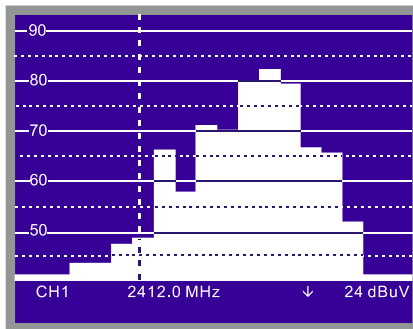
Figure 54.- Wi-Fi band spectrum representation.
