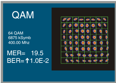
Figure 27.- Signal with noise and levels IQ nonbalanced.
