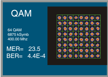
Figure 25.- Constellation Diagram of a signal with noise.
