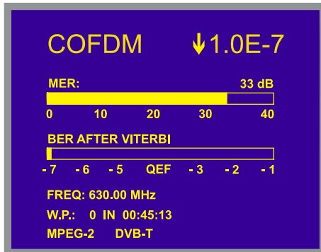
Figure 18.- MER measuring screen for COFDM-modulated signals.
