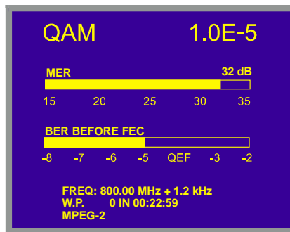
Figure 13.- BER measuring screen for QAM-modulated signals.
