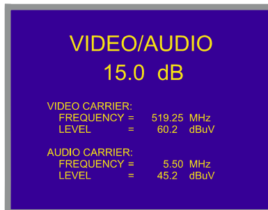
Figure 9.- Video/Audio rate measurement
