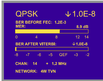
Figure 21.- MER measuring screen for QPSK-modulated signals.
