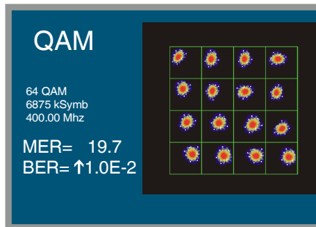
Figure 29.- QAM -Constellation Zoom function.
