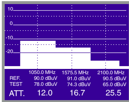
Figure 52.- Attenuation measurements in a plug.
