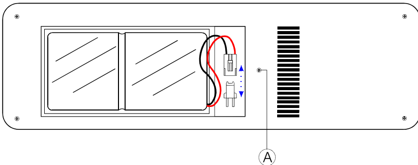
Figure 76.- Battery compartment.
