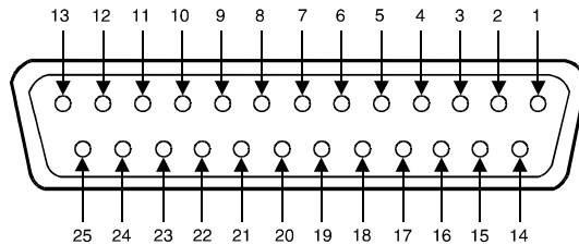
Figure 71.- Parallel Connector (LVDS D-25). External view.
