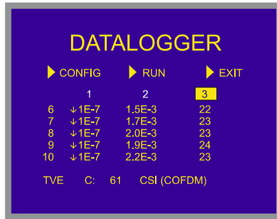
Figure 48.- Automatic measurements of the digital signals parameters.
