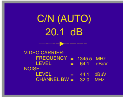
Figure 10.- Carrier-to-noise ratio measurement (Auto mode).
