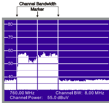
Figure 62.- Channel power measurement in Spectrum Mode.
