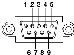
Figure 67.- Connector RS-232C PROLINK-4/4C Premium . Pins numbering.
