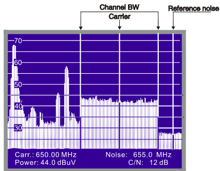
Figure 61.- Carrier to Noise measurement in Spectrum mode (digital channel).
