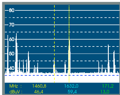
Figure 60.- Spectrum Analyser mode with two tuning markers.
