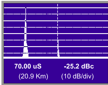
Figure 31b.- DVB-T COFDM signal impulsive response.
