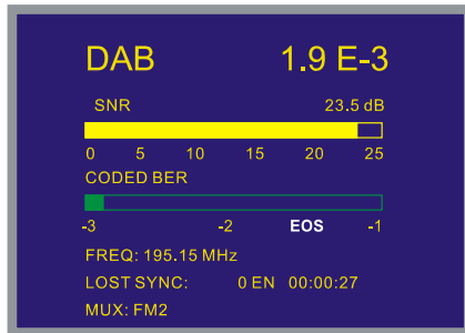
Figure 32.- DAB signal detection.
