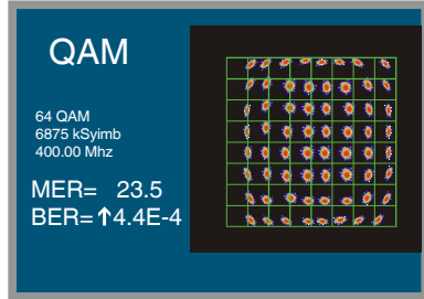
Figure 26.- Signal showing nonbalanced IQ levels.
