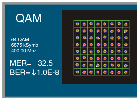
Figure 24.- Constellation Diagram of a DVB-64 QAM fair digital signal.
