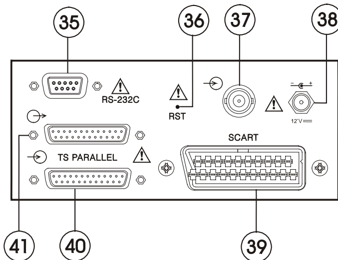
Figure 3.- Side panel connections.
