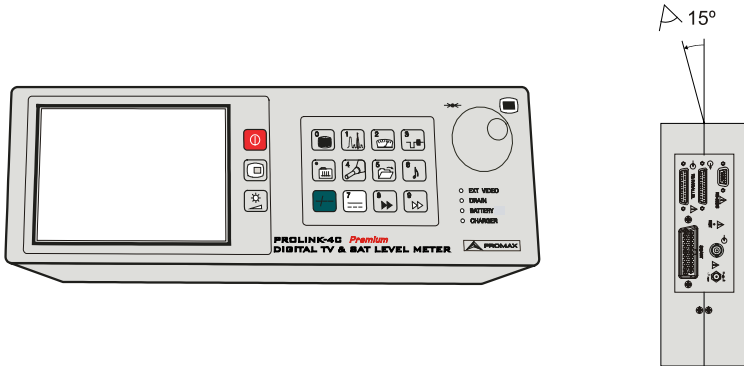
Figure 75.- Optimum viewing of the screen.
