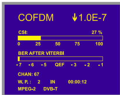
Figure 17.- Signalling two MPEG-2 signal cuts with a total length of 12 seconds.
